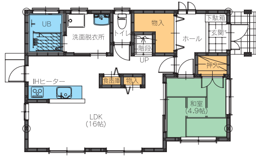
■ 1st Floor 60.25㎡
