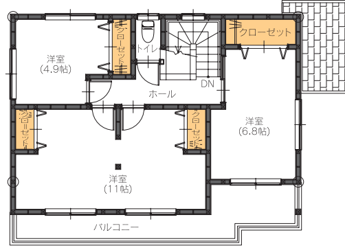
■ 2nd Floor 58.75㎡
